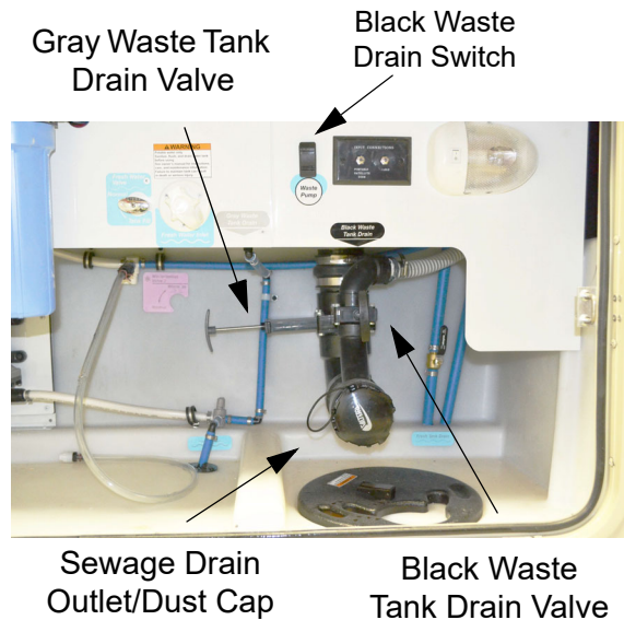
Holding Tank Drain Valves (Model 27PE Only - Located in water service center on driver side of motorhome)
