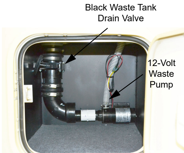
Black Holding Tank Waste Pump (Model 27PE Only - Located inside a passenger compartment)
