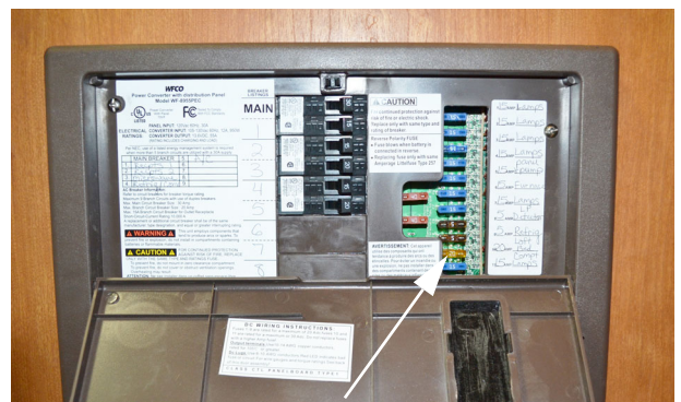
House 12-Volt Fuses (Located on Power Converter) -Typical View
